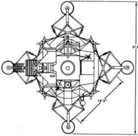
LEM is 31 feet or 9.5 metres at the widest.
